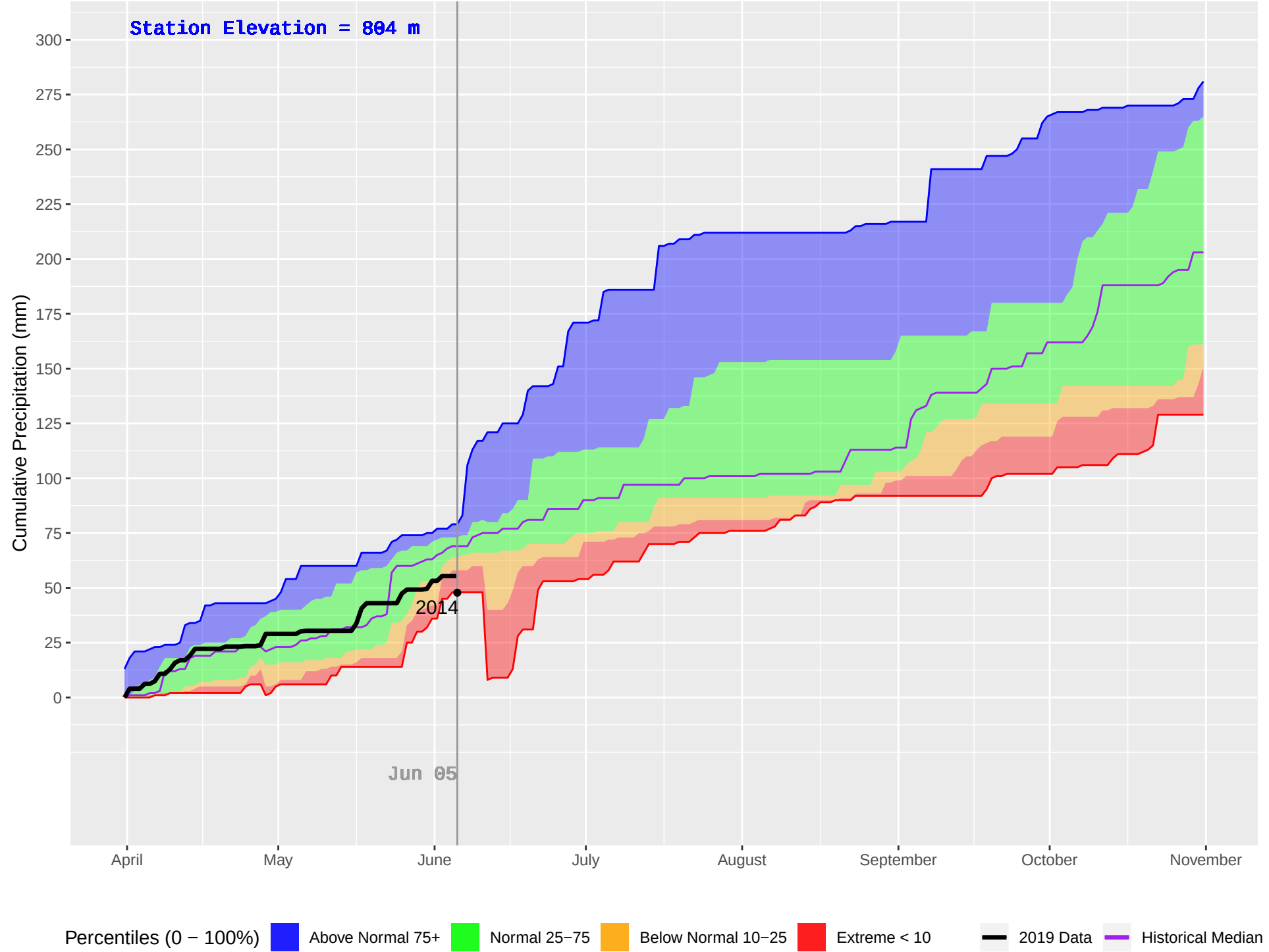
KOOCANUSA (1075) : Historical (2010–2018), Current (2019) Daily Cumulative Precipitation
