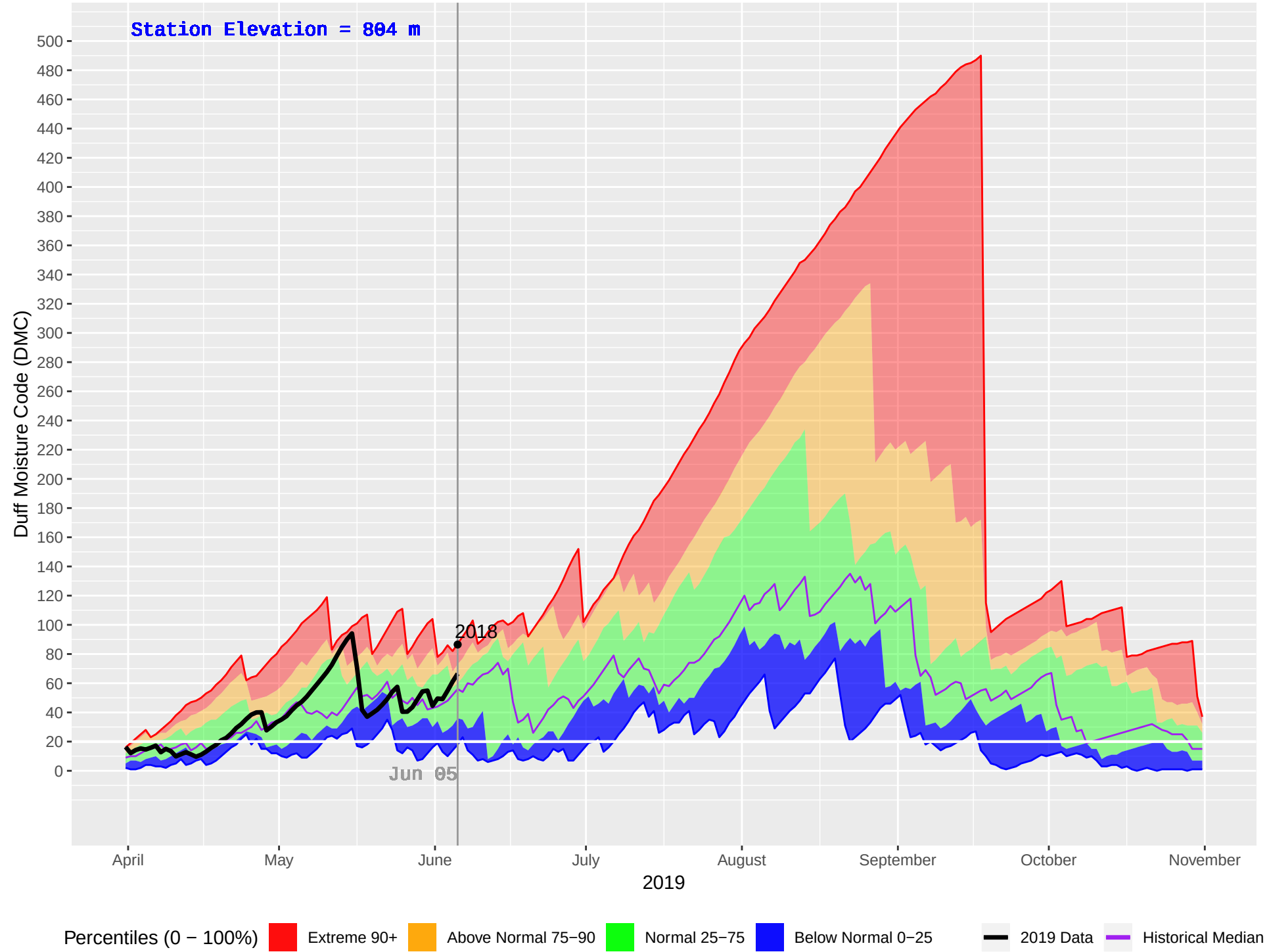
KOOCANUSA (1075) : Historical (2010–2018), Current (2019) Daily Duff Moisture Code (DMC)
