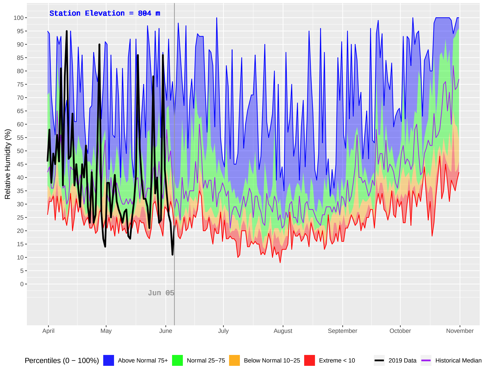
KOOCANUSA (1075) : Historical (2010–2018) and Current (2019) Daily Relative Humidity
