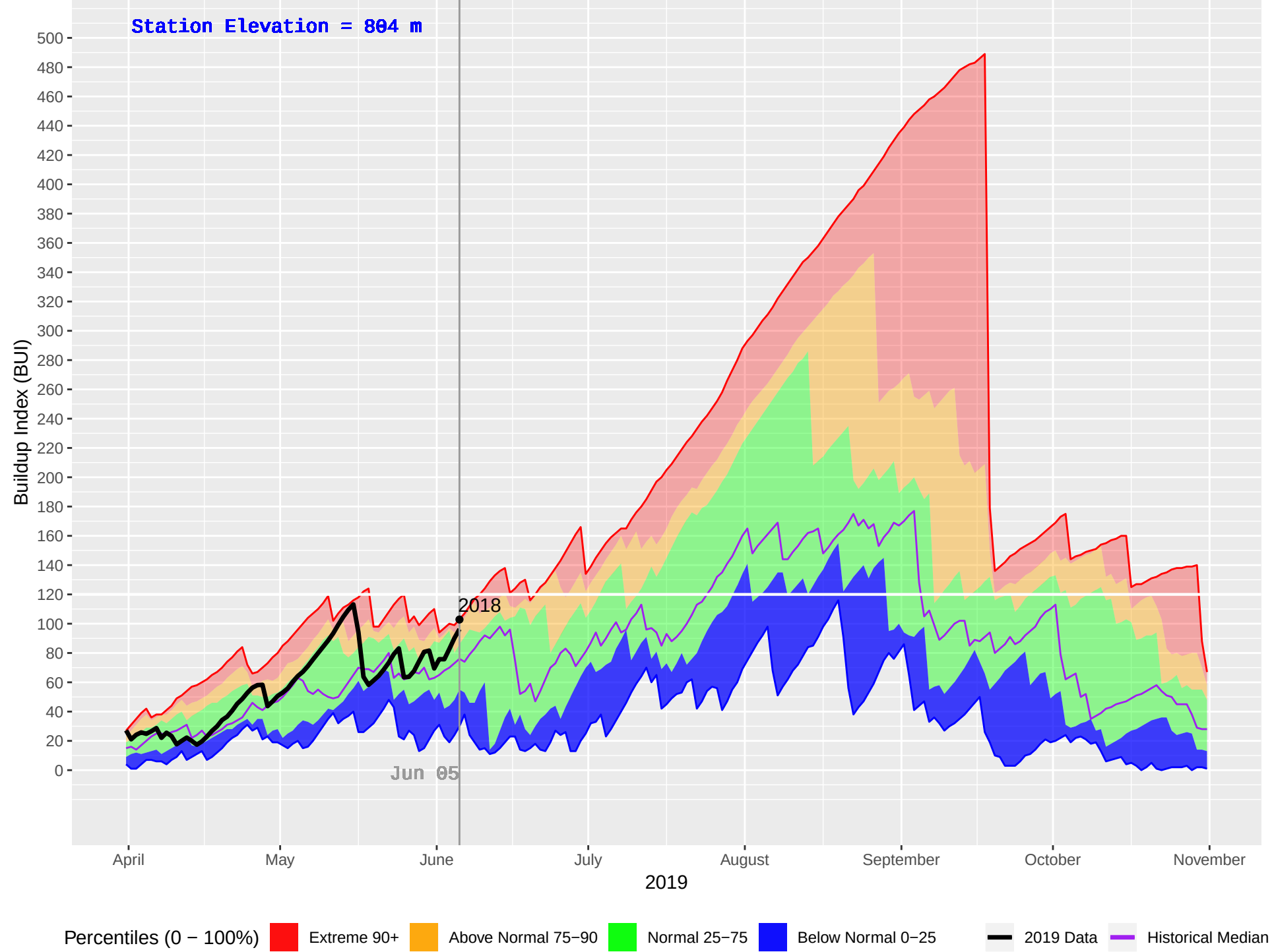
KOOCANUSA (1075) : Historical (2010–2018), Current (2019) Daily Buildup Index (BUI)
