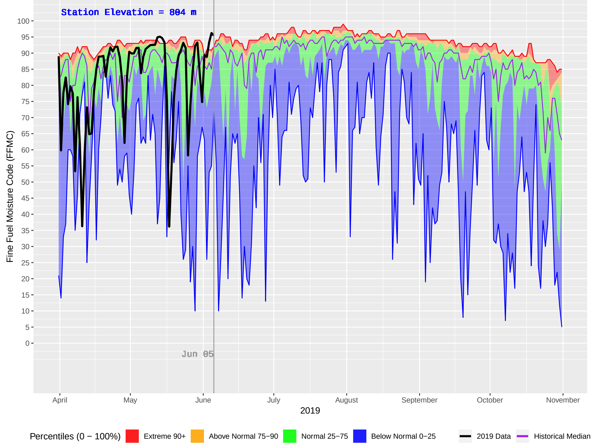
KOOCANUSA (1075) : Historical (2010–2018) and Current (2019) Daily Fine Fuel Moisture Code (FFMC)
